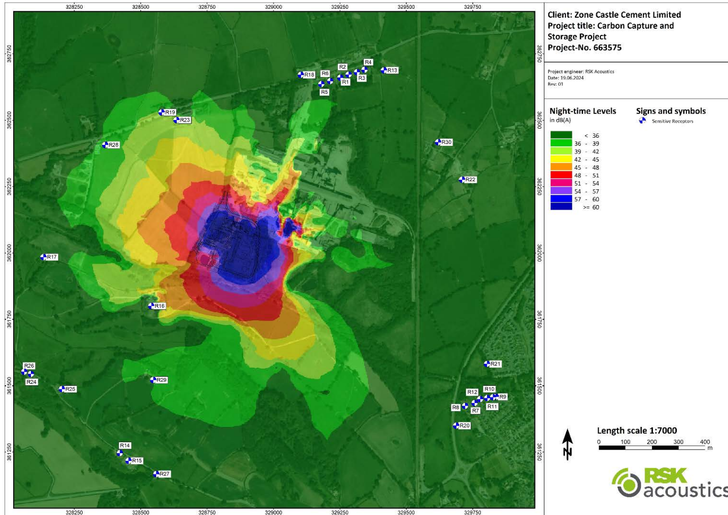
Figure 2 Contour Plot Night-time
