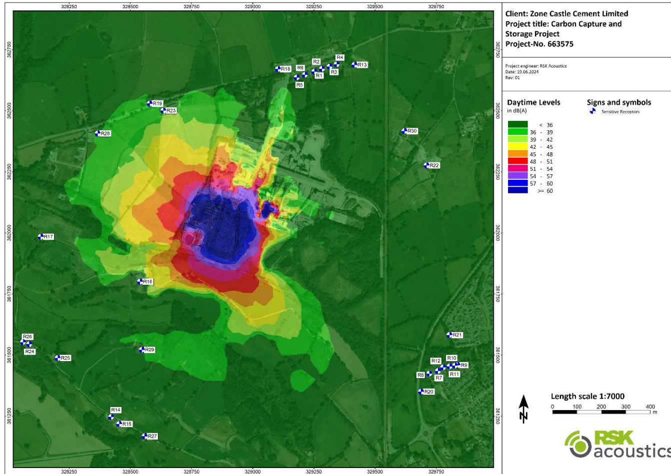
Figure 1 Contour Plot Day-time
